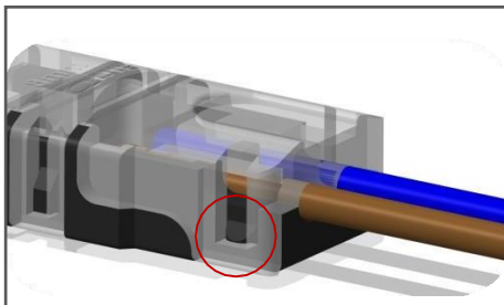
You will hear a "click sound" after you press the cover into the locking system
